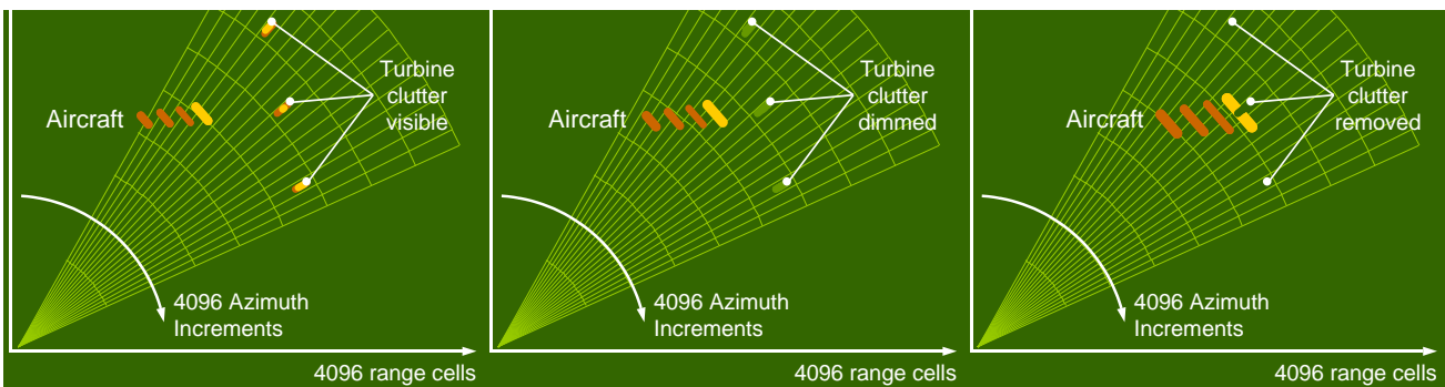
Primary Radar, perceives the world in terms of range and azimuth cells. If a target appears in a range-azimuth cell, then the cell is illuminated, otherwise it is empty.
